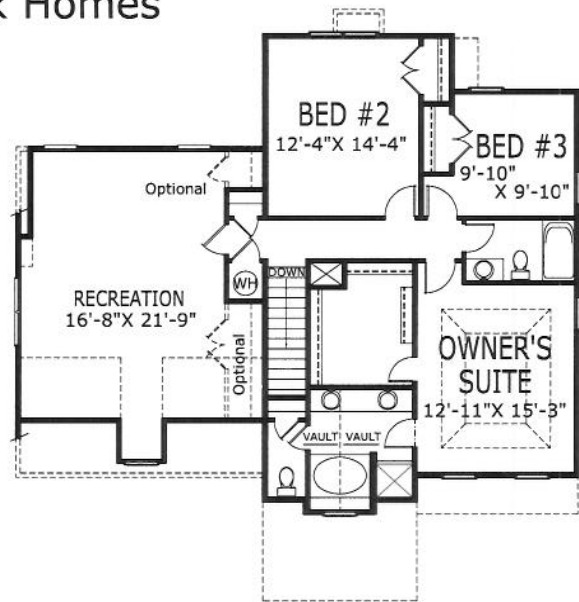
SECOND FLOOR (ELEVATION 0)
